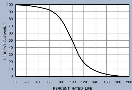
Lamp Mortality Curve
